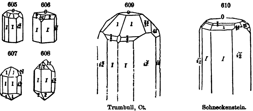
Trumbull, Ct.
